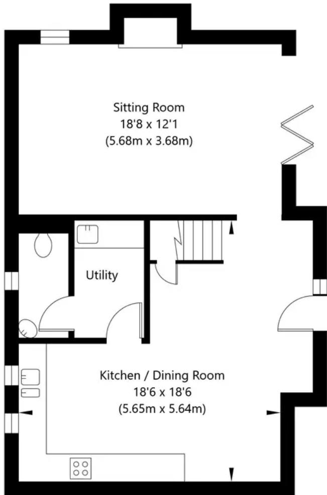
Ground Floor GROSS INTERNAL FLOOR AREA APPROX. 610 SQ FT / 56.71 SQ M
